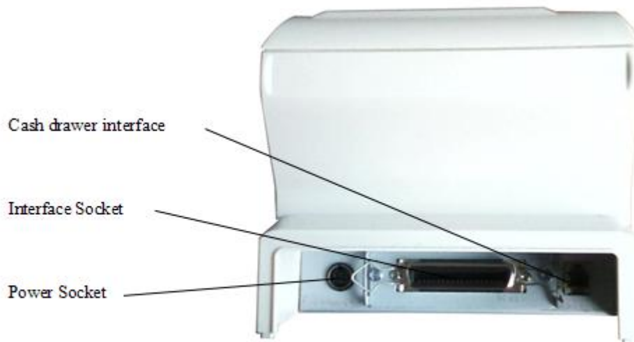
Fig.2-1 Printer Appearance
